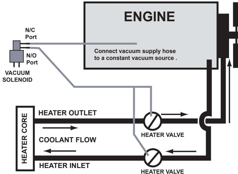
Diagram 3 - Heater Hose Flow
