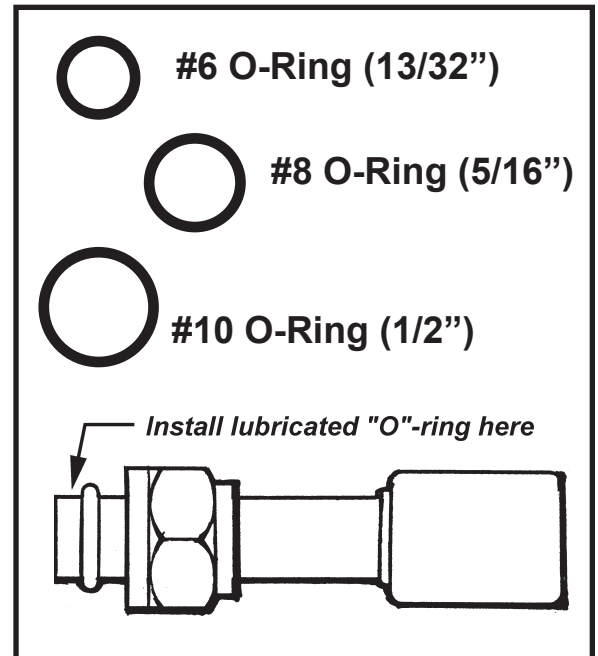
Diagram #2 - O-Ring Seals
