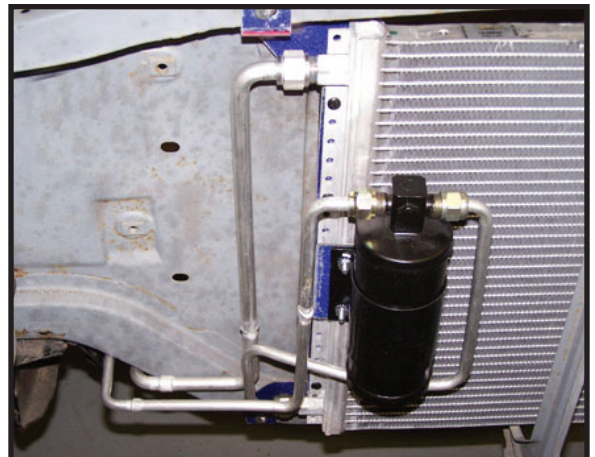
Photo 12 - Drier & Tubes
