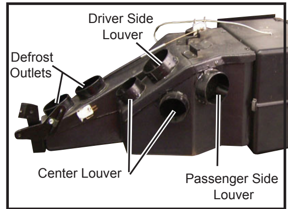
Photo 10 - Unit Outlet
